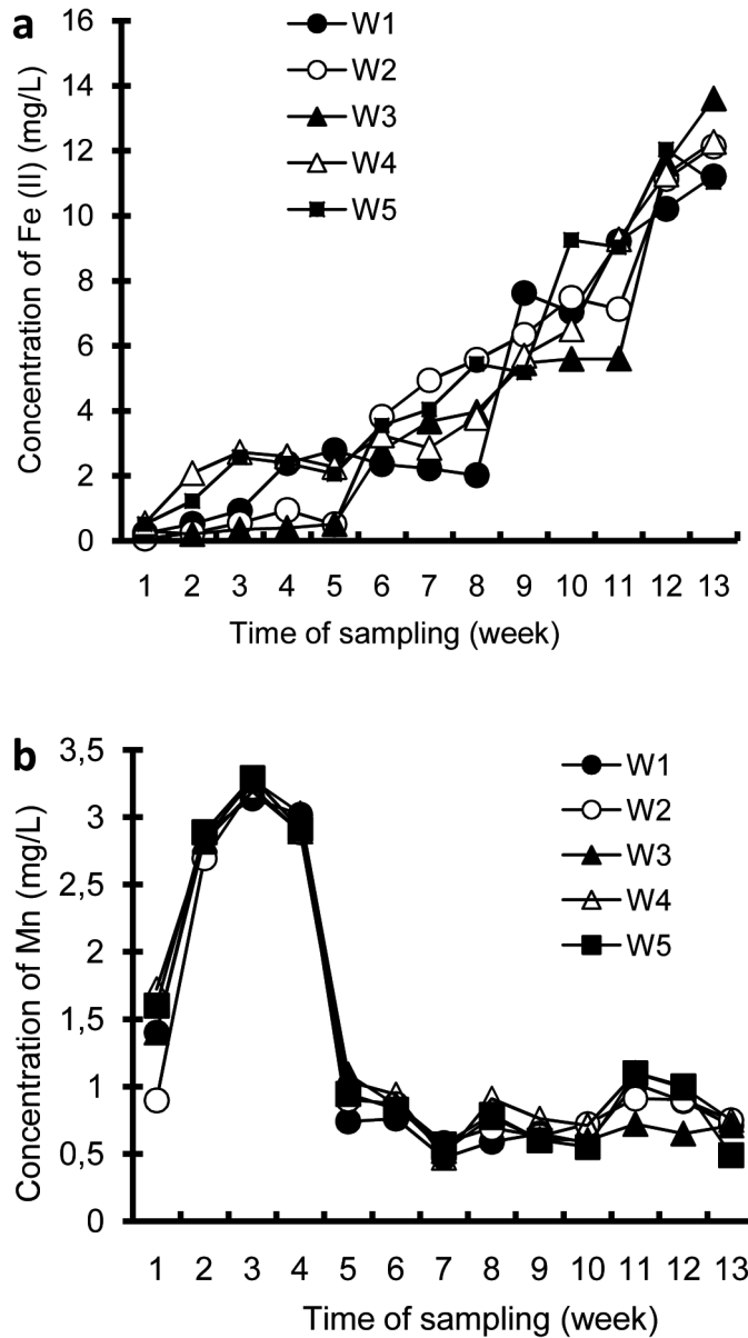
Fig.2: The temporal changes of the iron and manganese concentrations in the soil extract a) Fe^{2+} concentrations increased slowly with time but increased markedly after water was drained out. Weekly data showed no differences; (b) Mn concentrations increased markedly after flooding but it then decreased again to a stable level.
